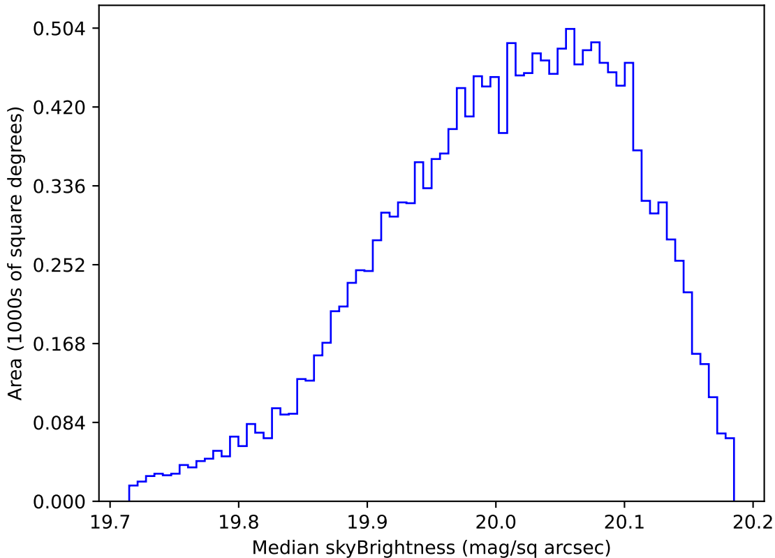
too_elab_r16_d2_ugrizy_v3.4_10yrs WFD i band: Median skyBrightness
