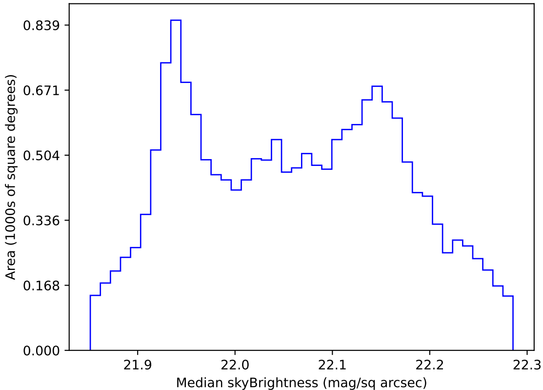
too_elab_r16_d2_ugrizy_v3.4_10yrs WFD g band: Median skyBrightness
