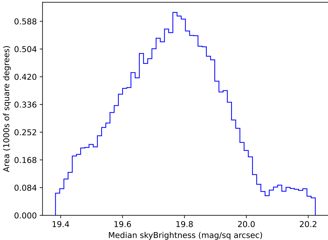
too_elab_r16_d2_ugrizy_v3.4_10yrs WFD all bands: Median skyBrightness
