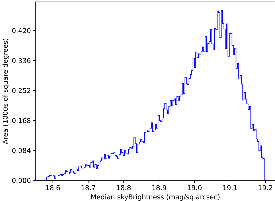
too_elab_r16_d2_ugrizy_v3.4_10yrs All sky z band: Median skyBrightness
