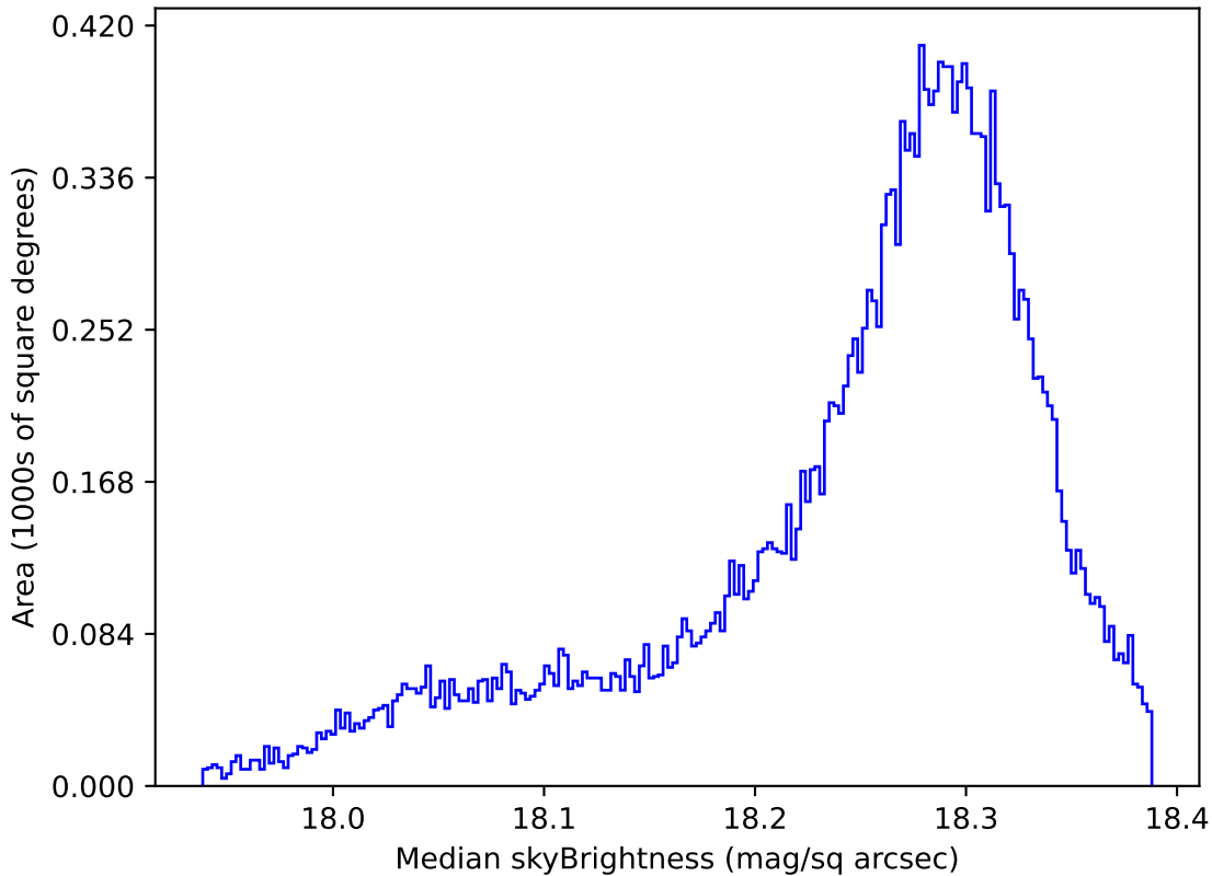
too_elab_r16_d2_ugrizy_v3.4_10yrs All sky y band: Median skyBrightness
