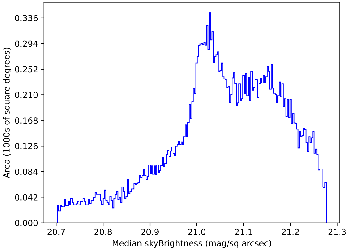
too_elab_r16_d2_ugrizy_v3.4_10yrs All sky r band: Median skyBrightness
