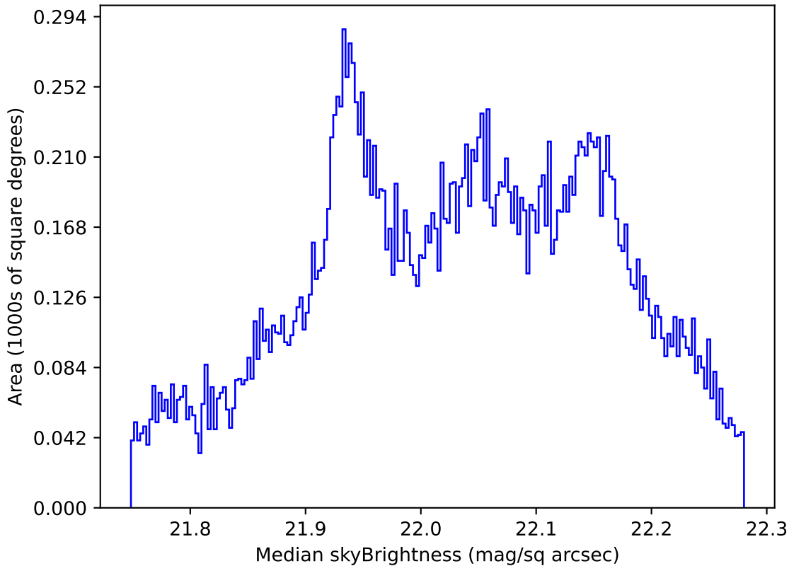
too_elab_r16_d2_ugrizy_v3.4_10yrs All sky g band: Median skyBrightness
