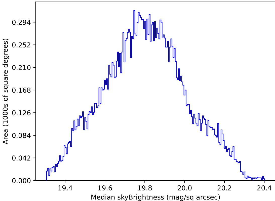
too_elab_r16_d2_ugrizy_v3.4_10yrs All sky all bands: Median skyBrightness
