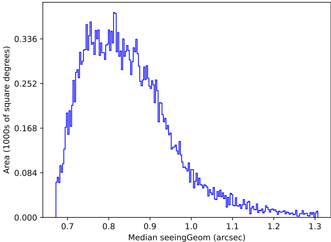
too_elab_r16_d2_ugrizy_v3.4_10yrs Yr 1 z band: Median seeingGeom
