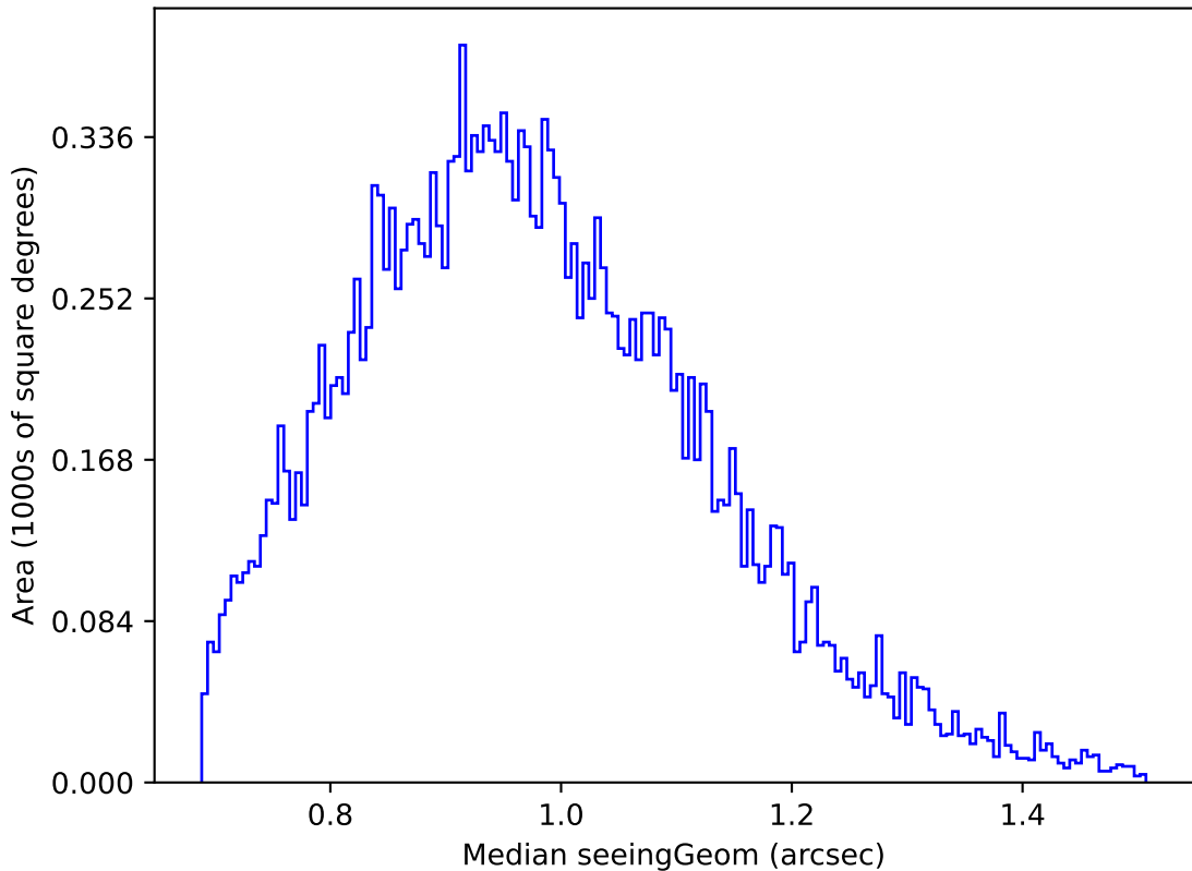
too_elab_r16_d2_ugrizy_v3.4_10yrs Yr 1 u band: Median seeingGeom
