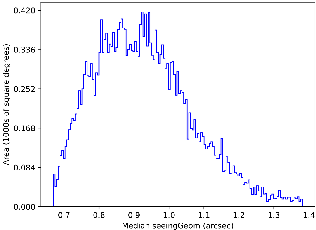
too_elab_r16_d2_ugrizy_v3.4_10yrs Yr 1 g band: Median seeingGeom
