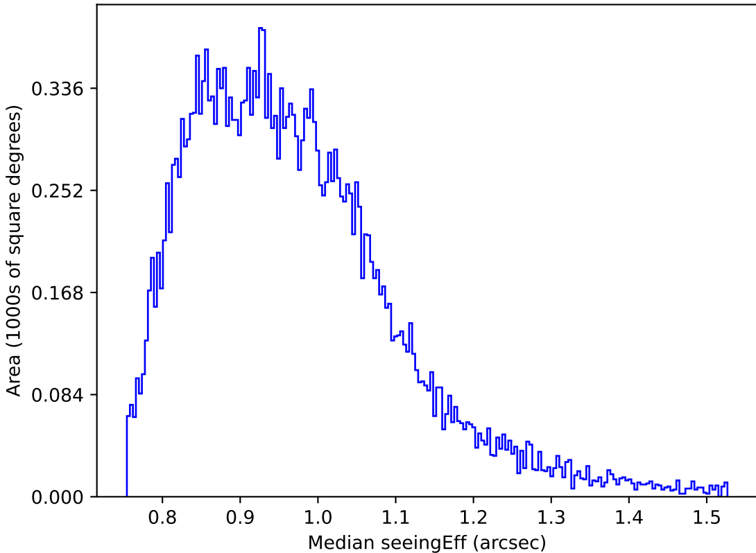
too_elab_r16_d2_ugrizy_v3.4_10yrs Yr 1 z band: Median seeingEff
