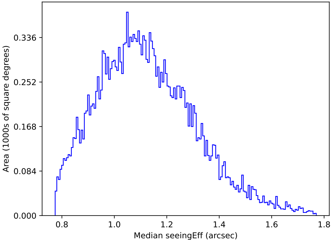
too_elab_r16_d2_ugrizy_v3.4_10yrs Yr 1 u band: Median seeingEff
