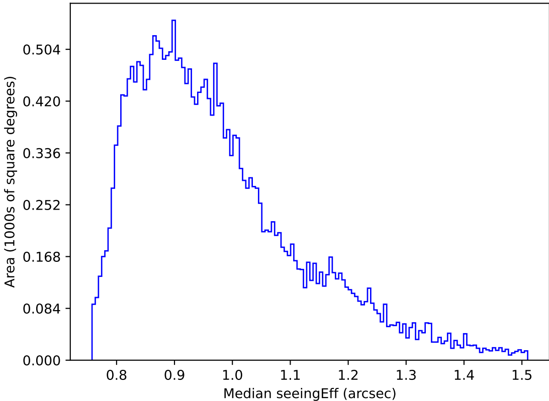
too_elab_r16_d2_ugrizy_v3.4_10yrs Yr 1 r band: Median seeingEff
