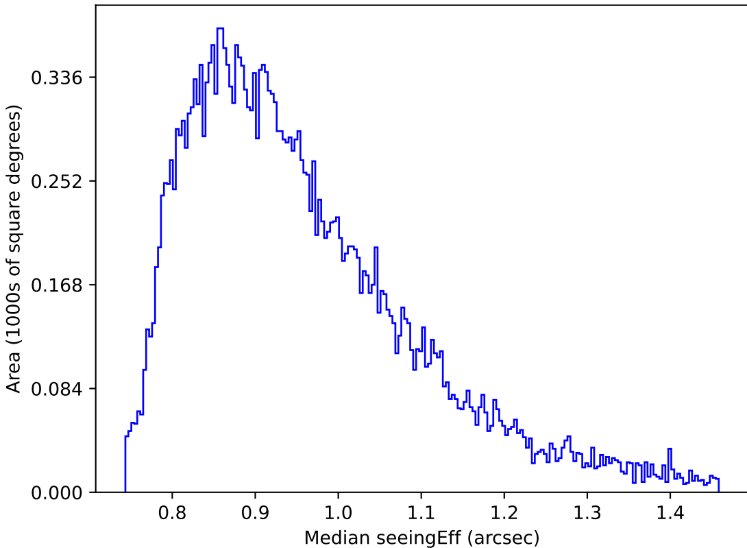
too_elab_r16_d2_ugrizy_v3.4_10yrs Yr 1 i band: Median seeingEff
