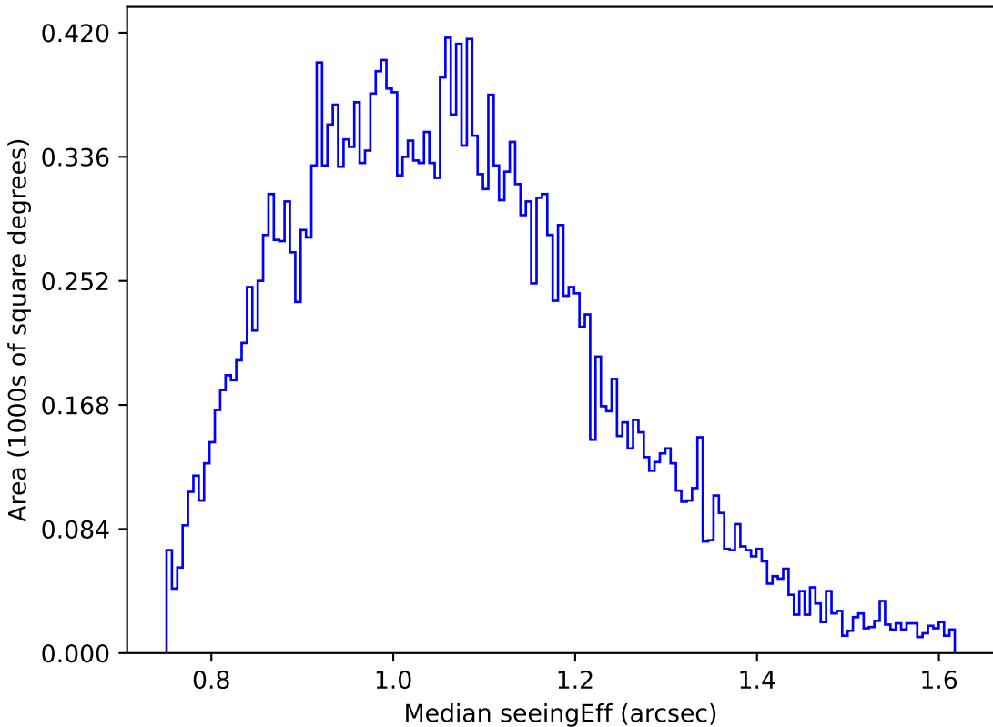
too_elab_r16_d2_ugrizy_v3.4_10yrs Yr 1 g band: Median seeingEff
