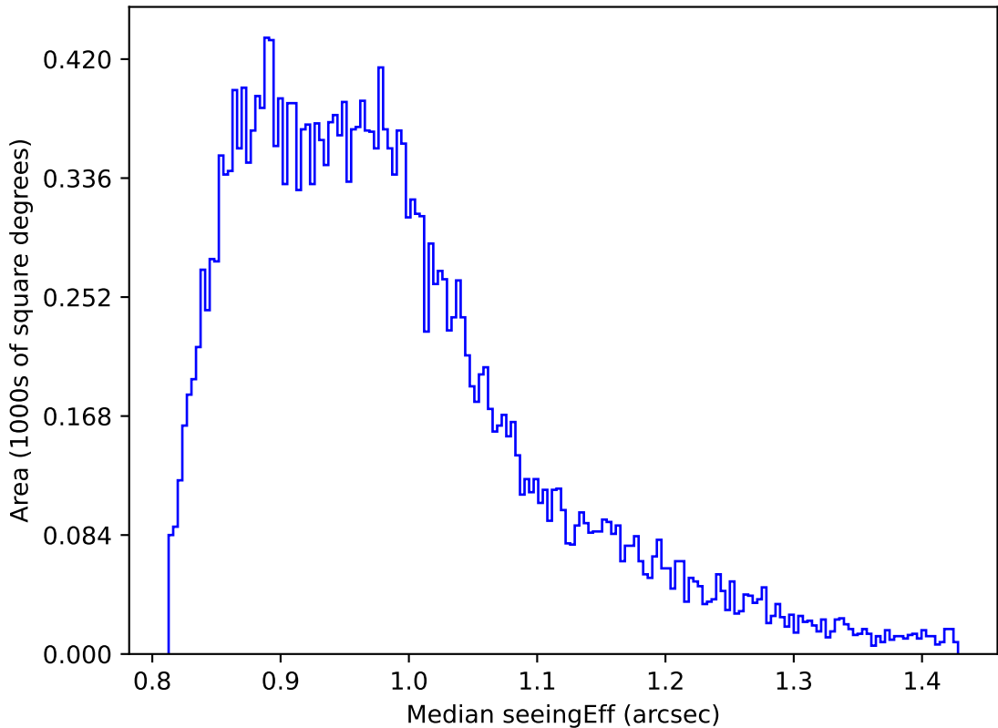
too_elab_r16_d2_ugrizy_v3.4_10yrs Yr 1 all bands: Median seeingEff
