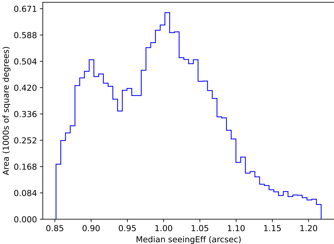
too_elab_r16_d2_ugrizy_v3.4_10yrs WFD i band: Median seeingEff
