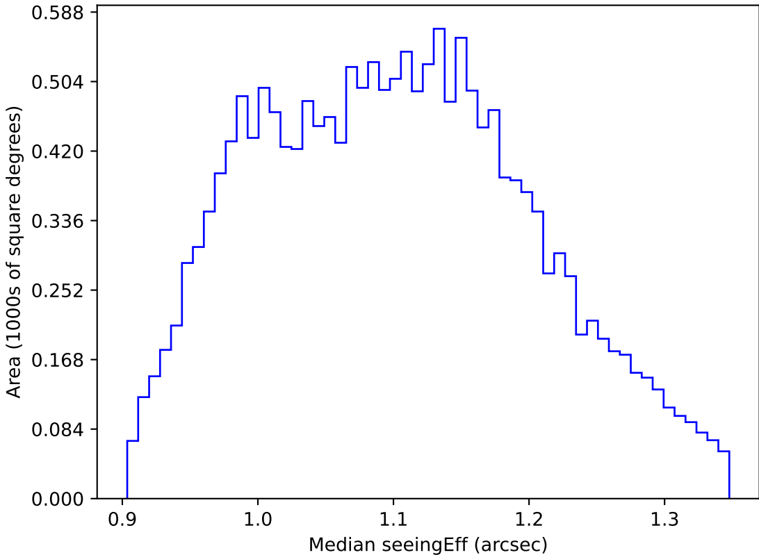
too_elab_r16_d2_ugrizy_v3.4_10yrs WFD g band: Median seeingEff
