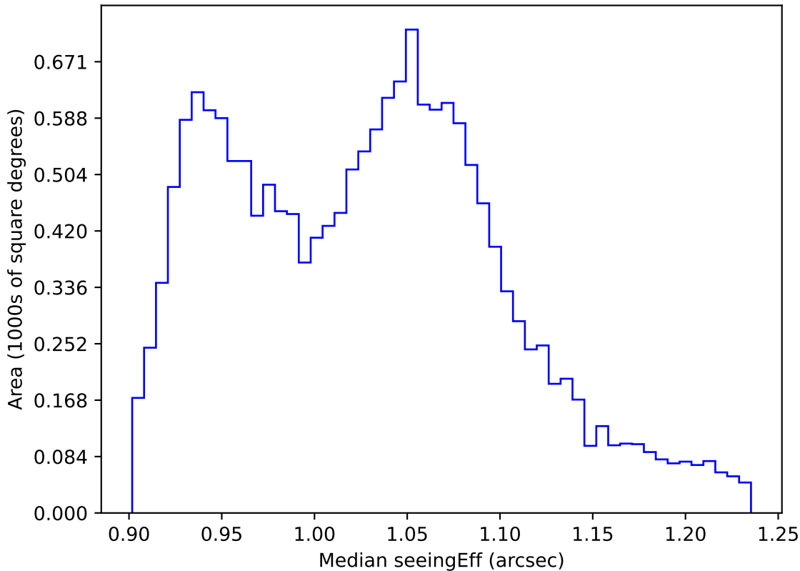
too_elab_r16_d2_ugrizy_v3.4_10yrs WFD all bands: Median seeingEff
