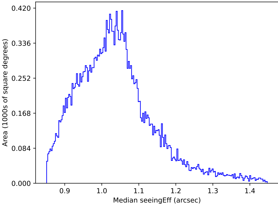
too_elab_r16_d2_ugrizy_v3.4_10yrs All sky z band: Median seeingEff
