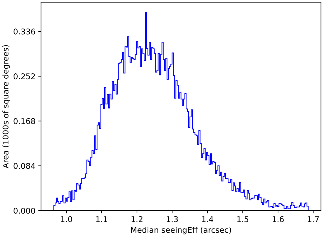
too_elab_r16_d2_ugrizy_v3.4_10yrs All sky u band: Median seeingEff
