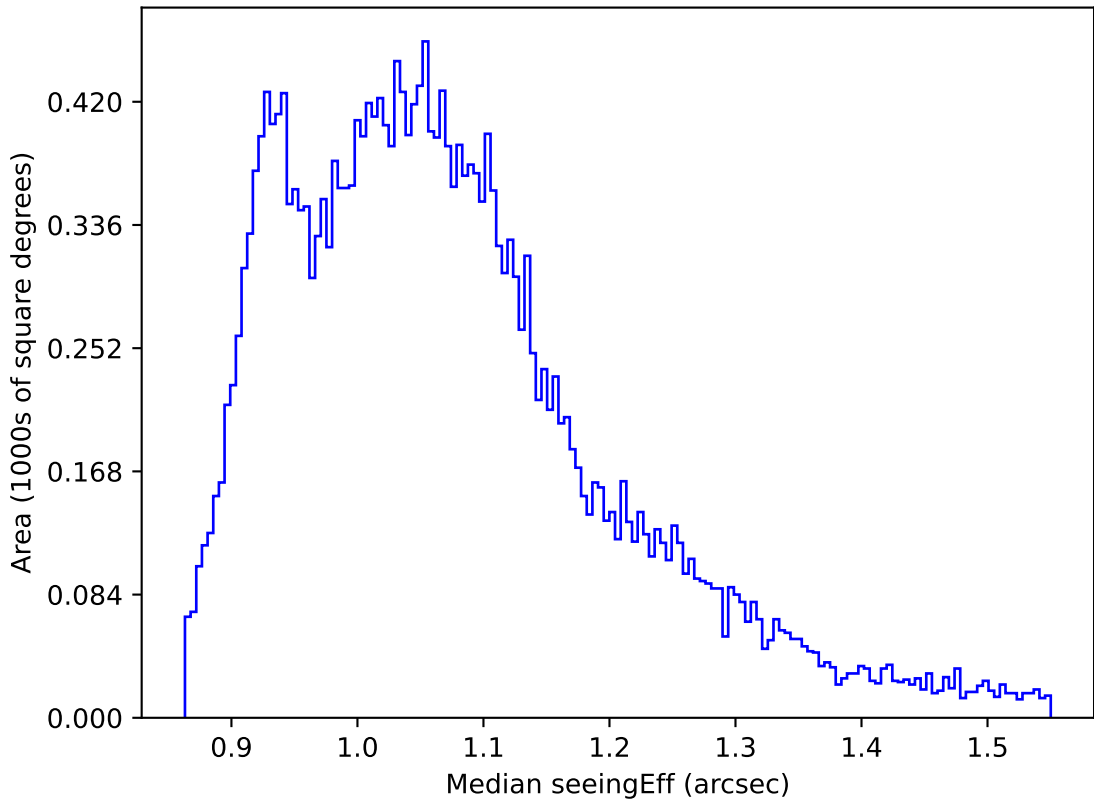
too_elab_r16_d2_ugrizy_v3.4_10yrs All sky r band: Median seeingEff
