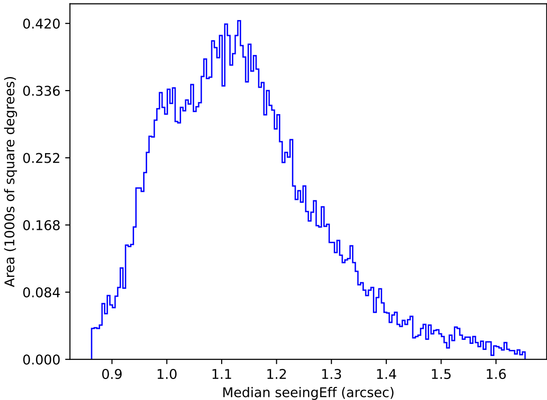
too_elab_r16_d2_ugrizy_v3.4_10yrs All sky g band: Median seeingEff
