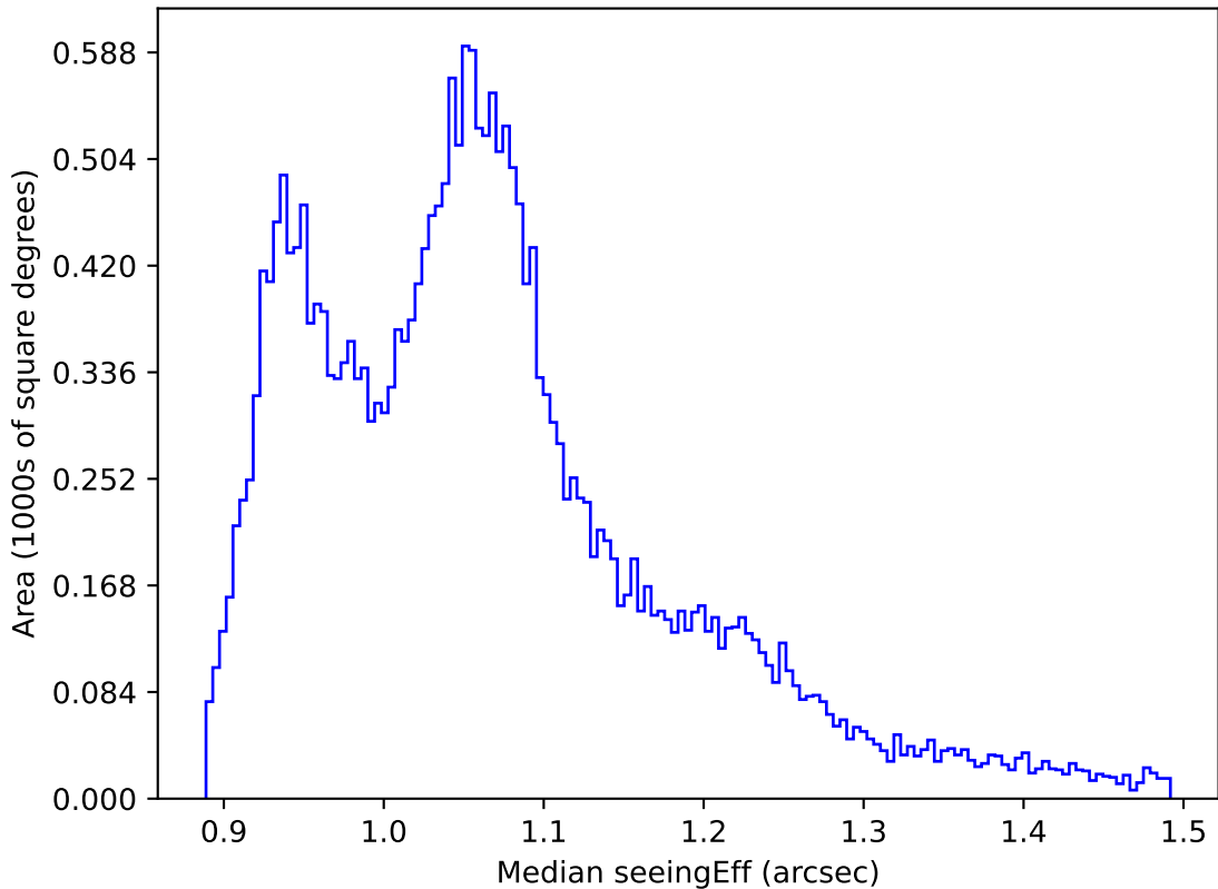
too_elab_r16_d2_ugrizy_v3.4_10yrs All sky all bands: Median seeingEff
