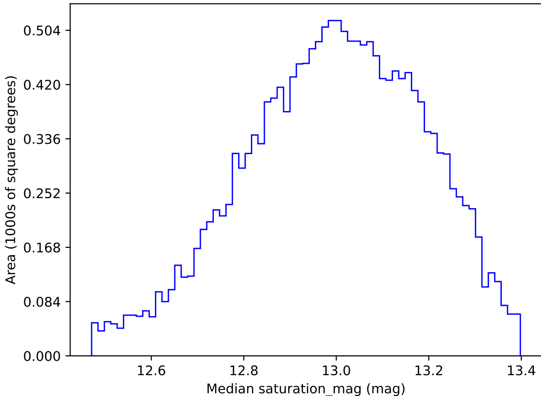
too_elab_r16_d2_ugrizy_v3.4_10yrs WFD u band: Median saturation_mag
