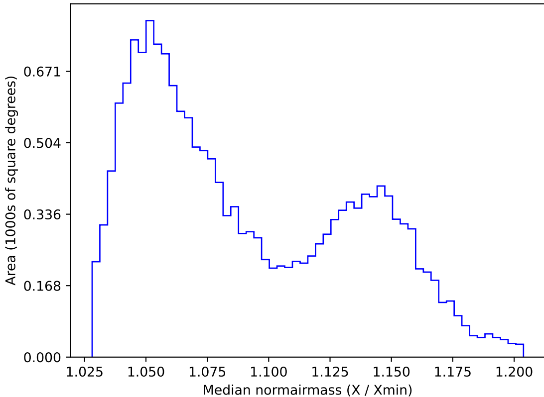
too_elab_r16_d2_ugrizy_v3.4_10yrs WFD y band: Median normairmass
