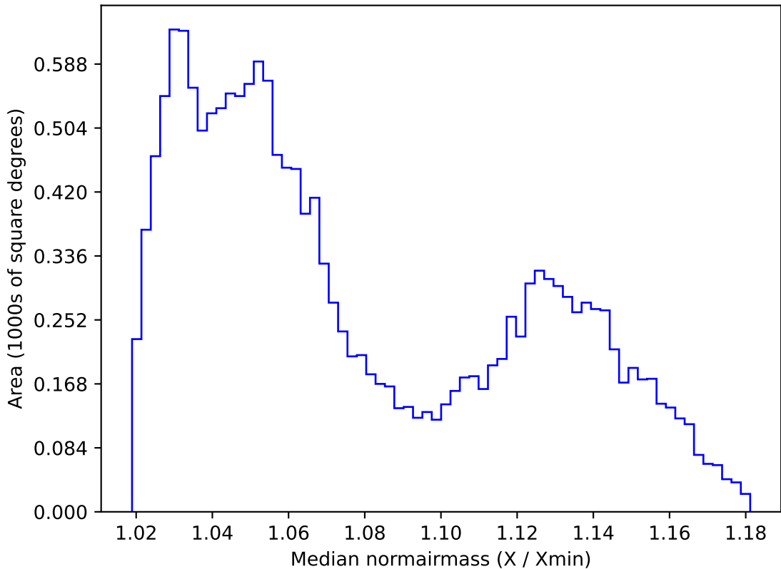
too_elab_r16_d2_ugrizy_v3.4_10yrs WFD i band: Median normairmass
