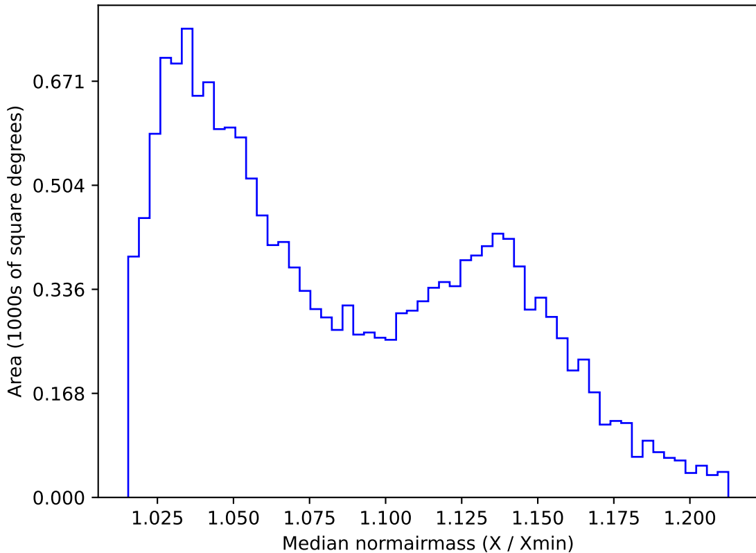
too_elab_r16_d2_ugrizy_v3.4_10yrs WFD g band: Median normairmass
