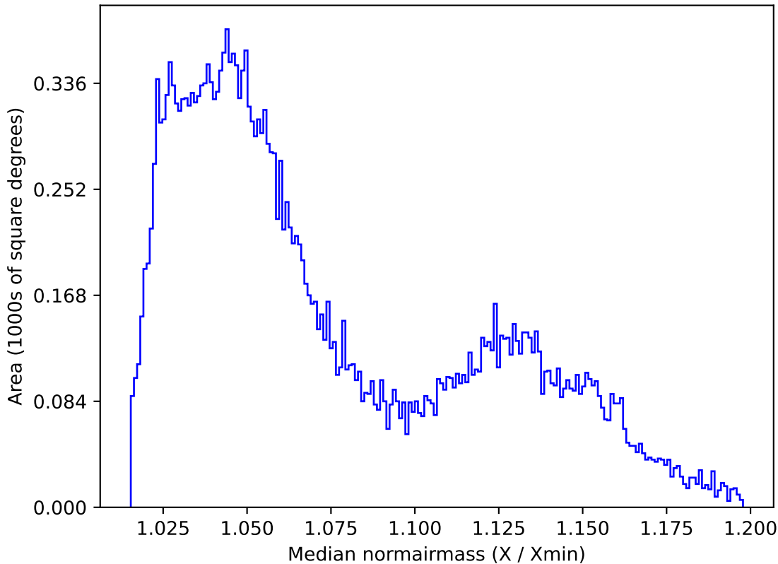
too_elab_r16_d2_ugrizy_v3.4_10yrs All sky r band: Median normairmass
