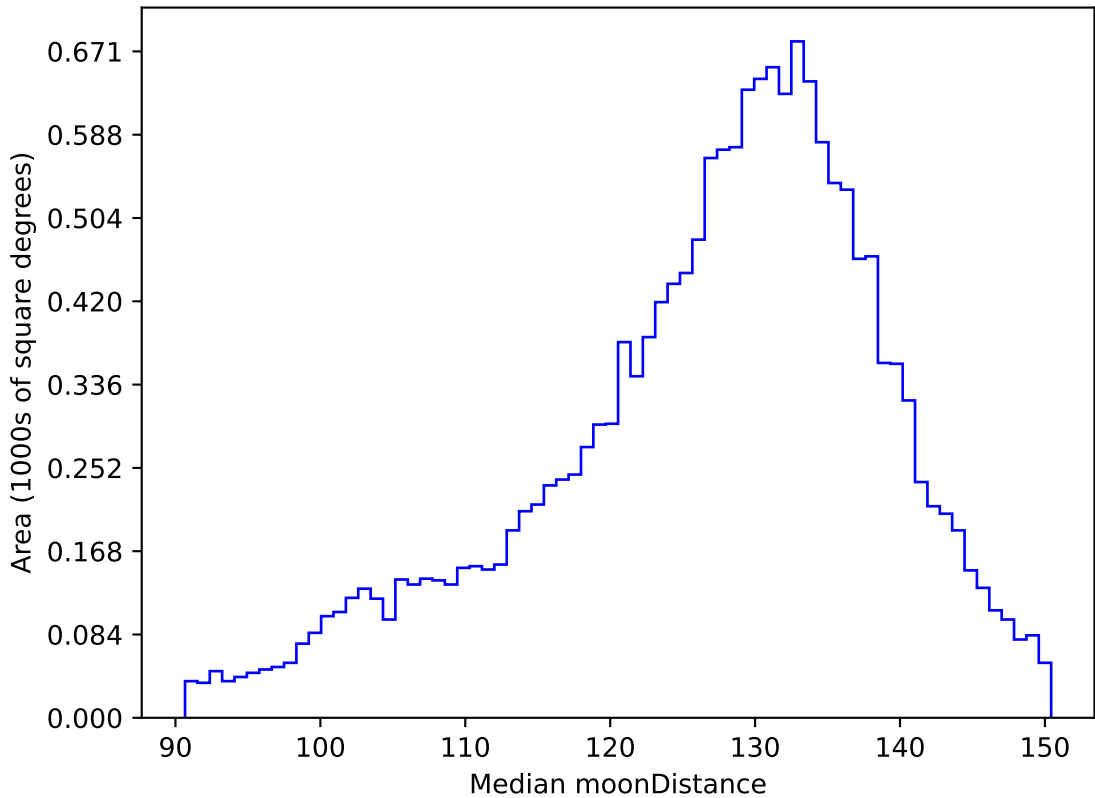
too_elab_r16_d2_ugrizy_v3.4_10yrs WFD u band: Median moonDistance
