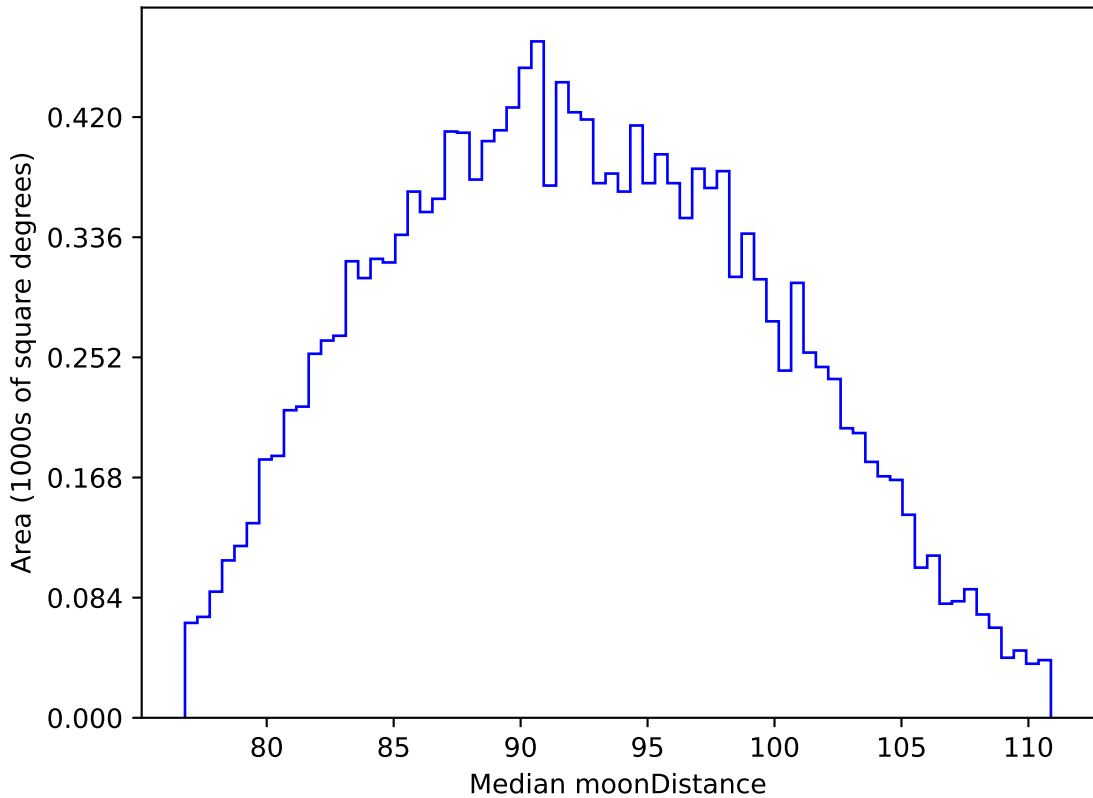
too_elab_r16_d2_ugrizy_v3.4_10yrs WFD i band: Median moonDistance
