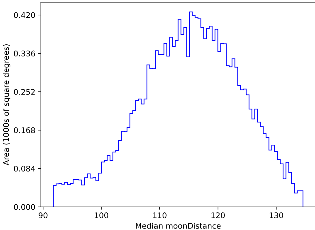
too_elab_r16_d2_ugrizy_v3.4_10yrs WFD g band: Median moonDistance
