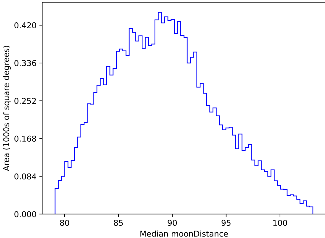
too_elab_r16_d2_ugrizy_v3.4_10yrs WFD all bands: Median moonDistance
