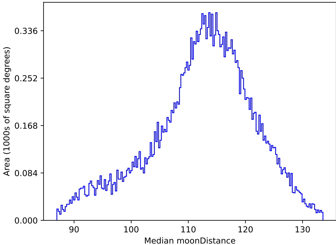
too_elab_r16_d2_ugrizy_v3.4_10yrs All sky r band: Median moonDistance
