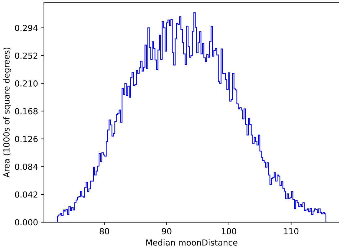
too_elab_r16_d2_ugrizy_v3.4_10yrs All sky i band: Median moonDistance
