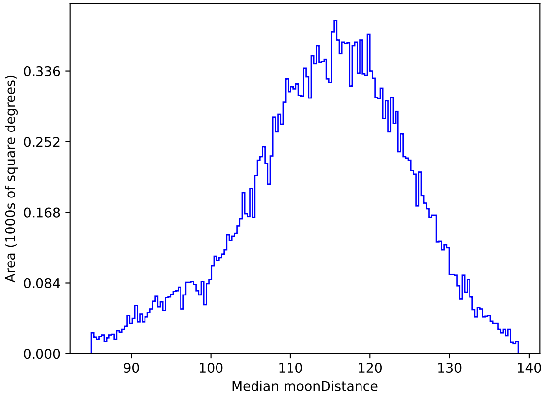
too_elab_r16_d2_ugrizy_v3.4_10yrs All sky g band: Median moonDistance
