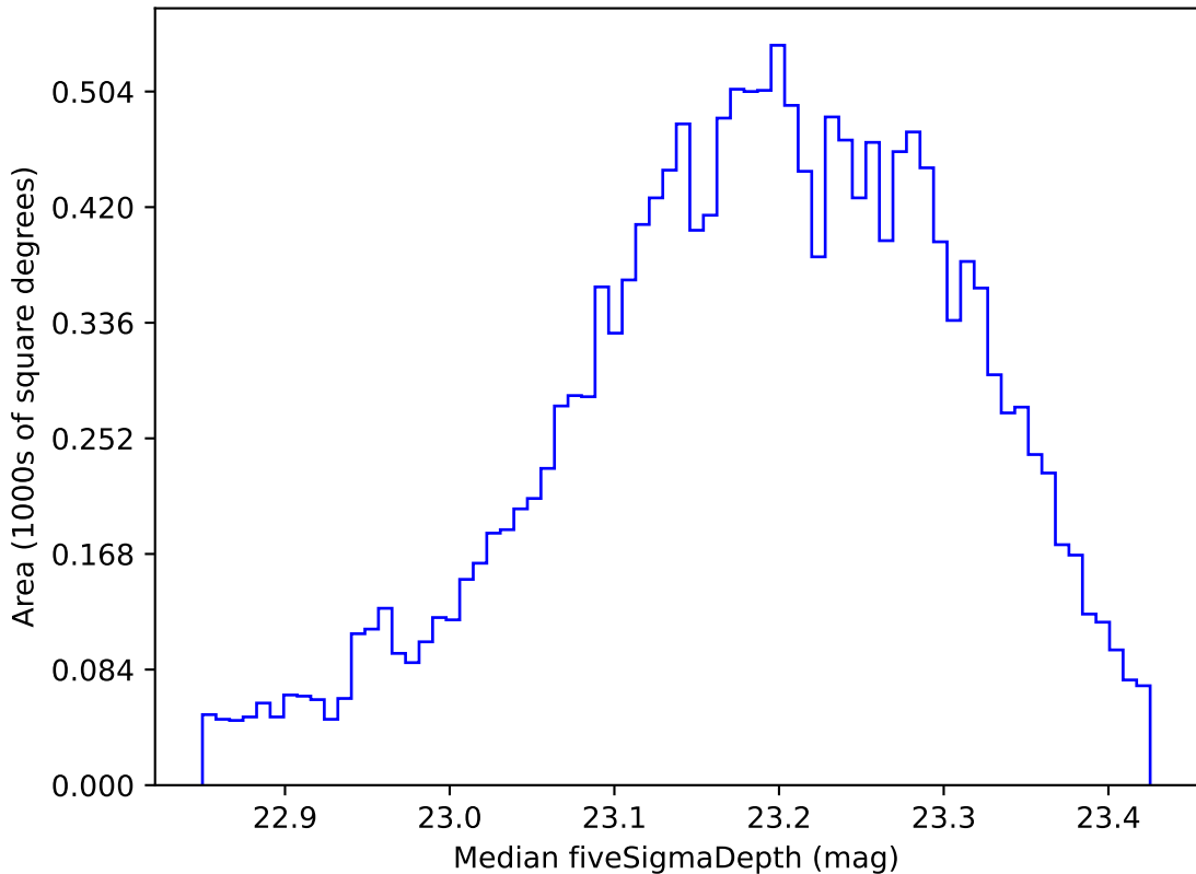
too_elab_r16_d2_ugrizy_v3.4_10yrs WFD u band: Median fiveSigmaDepth
