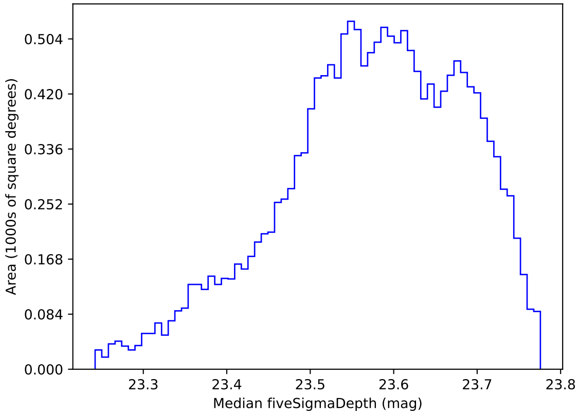
too_elab_r16_d2_ugrizy_v3.4_10yrs WFD i band: Median fiveSigmaDepth
