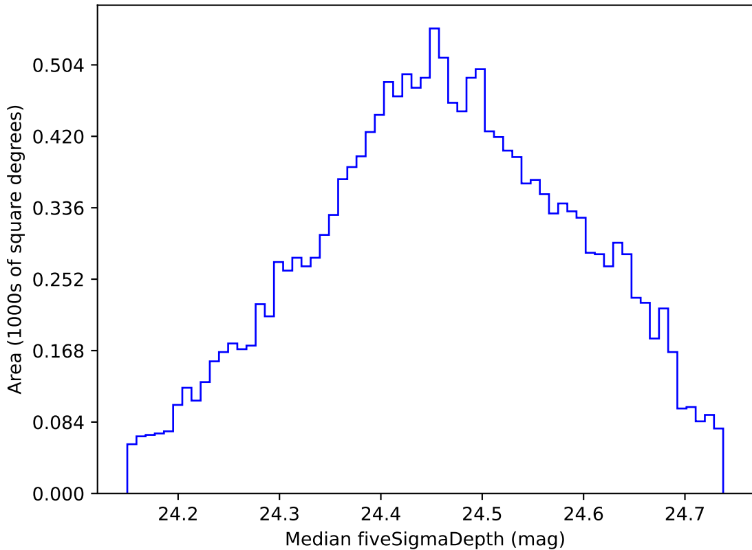
too_elab_r16_d2_ugrizy_v3.4_10yrs WFD g band: Median fiveSigmaDepth
