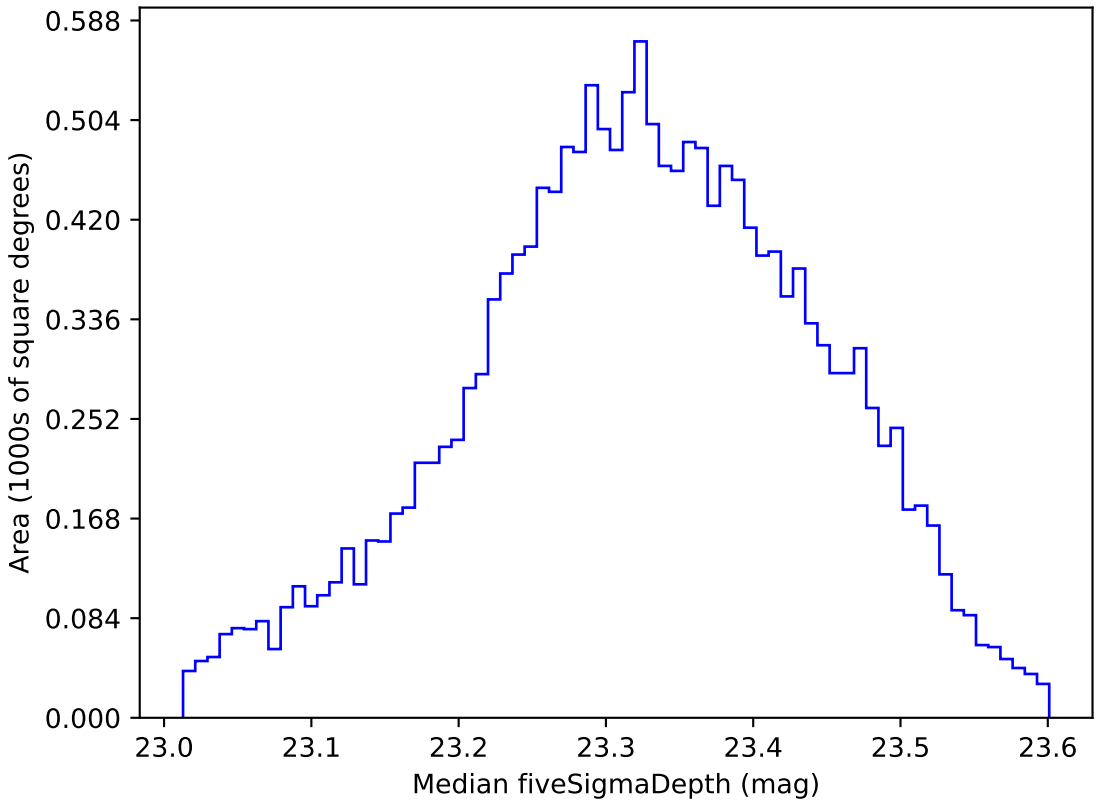
too_elab_r16_d2_ugrizy_v3.4_10yrs WFD all bands: Median fiveSigmaDepth
