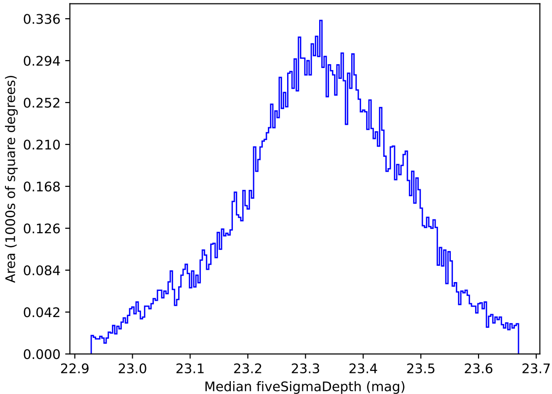
too_elab_r16_d2_ugrizy_v3.4_10yrs All sky all bands: Median fiveSigmaDepth
