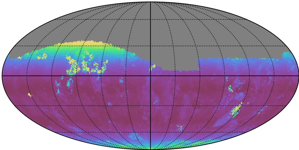
too_elab_r16_d2_ugrizy_v3.4_10yrs Yr 1 z band: Median airmass
