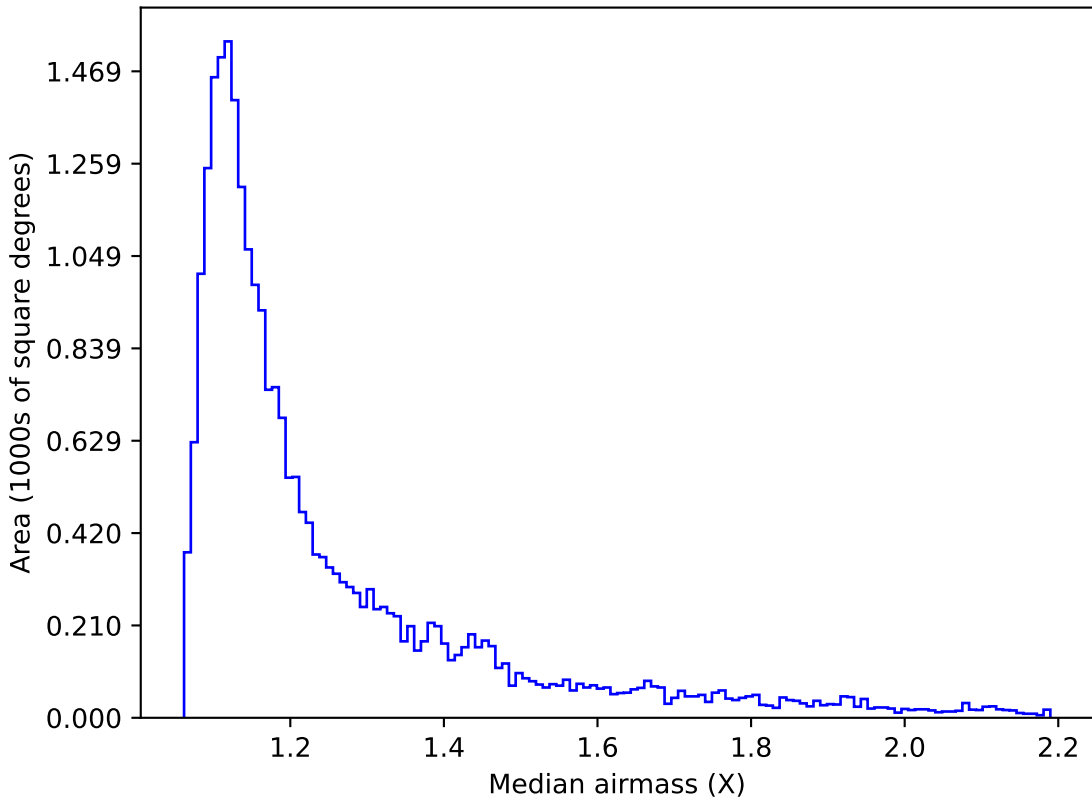
too_elab_r16_d2_ugrizy_v3.4_10yrs Yr 1 z band: Median airmass
