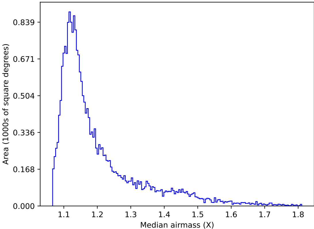
too_elab_r16_d2_ugrizy_v3.4_10yrs Yr 1 y band: Median airmass
