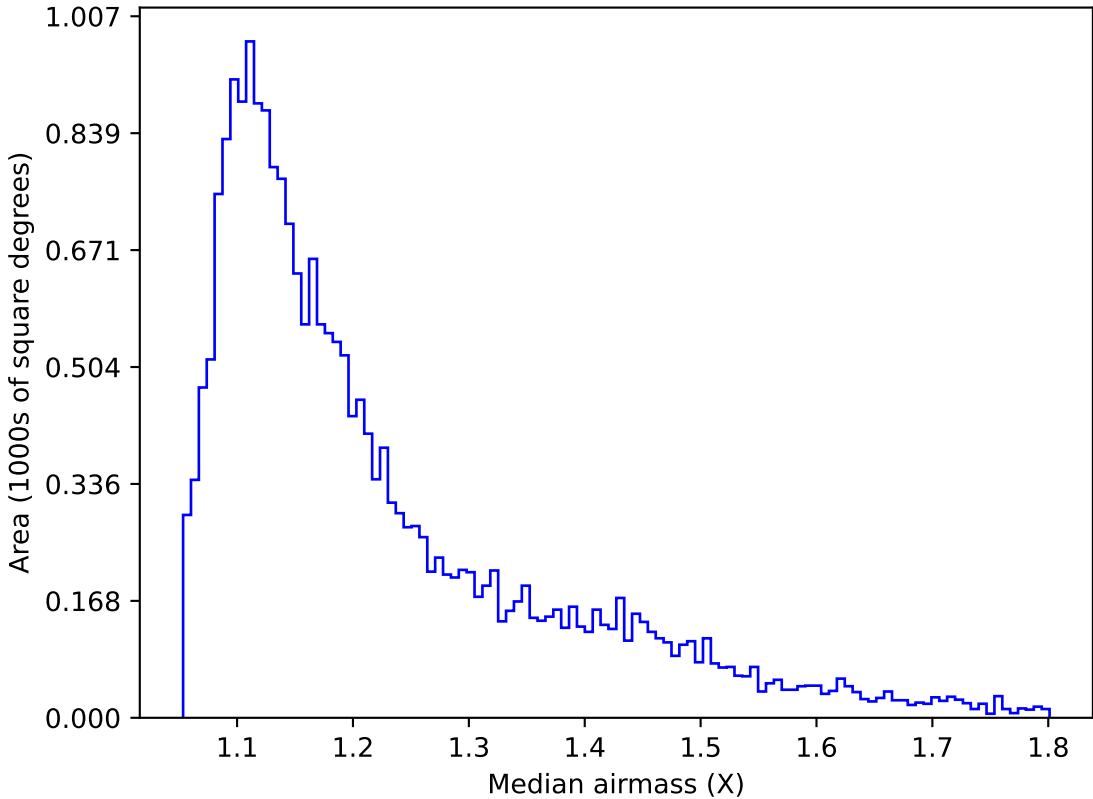
too_elab_r16_d2_ugrizy_v3.4_10yrs Yr 1 u band: Median airmass
