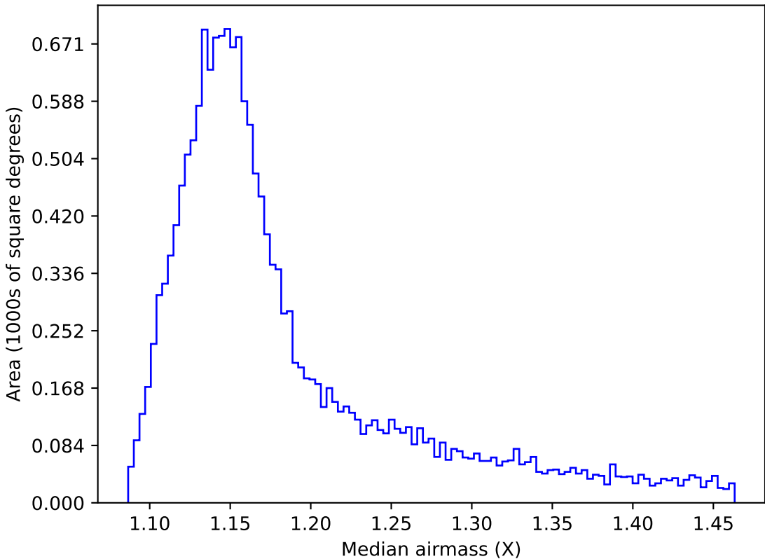
too_elab_r16_d2_ugrizy_v3.4_10yrs WFD z band: Median airmass
