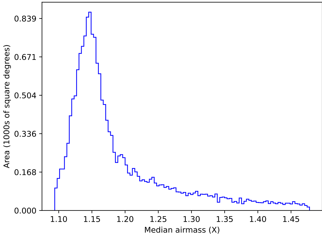
too_elab_r16_d2_ugrizy_v3.4_10yrs WFD y band: Median airmass
