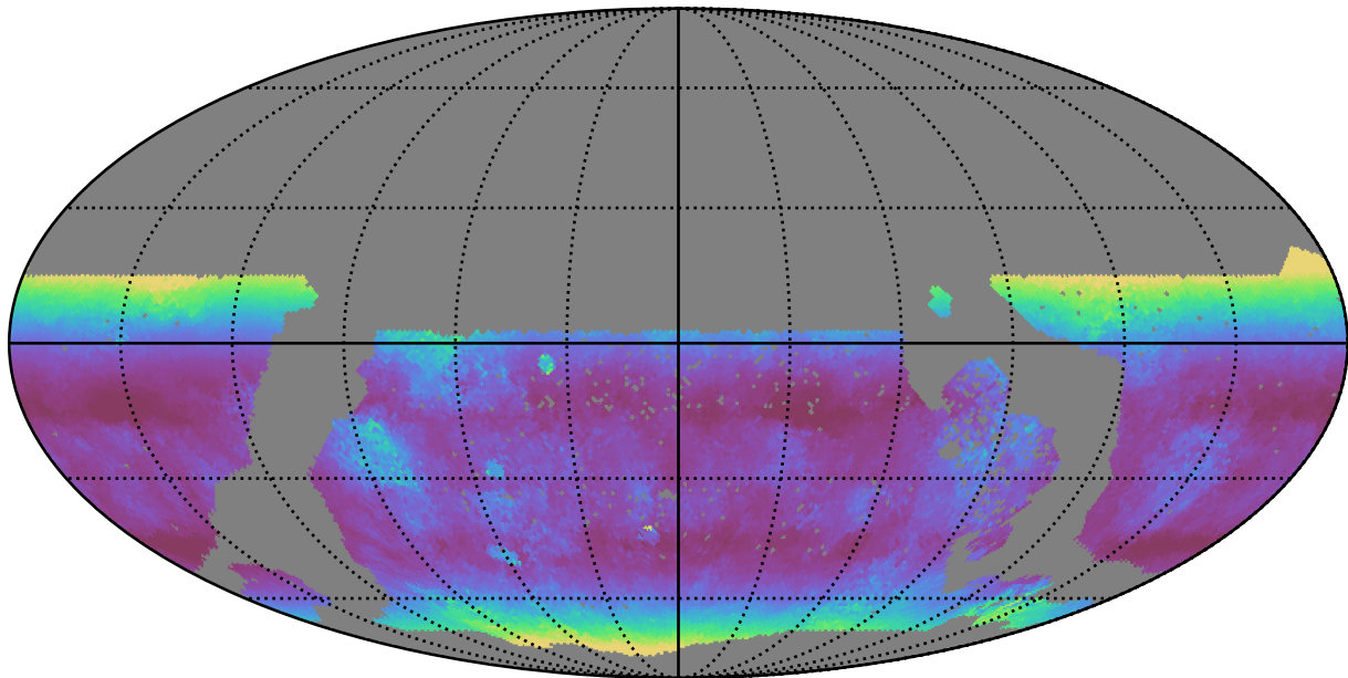
too_elab_r16_d2_ugrizy_v3.4_10yrs WFD u band: Median airmass
