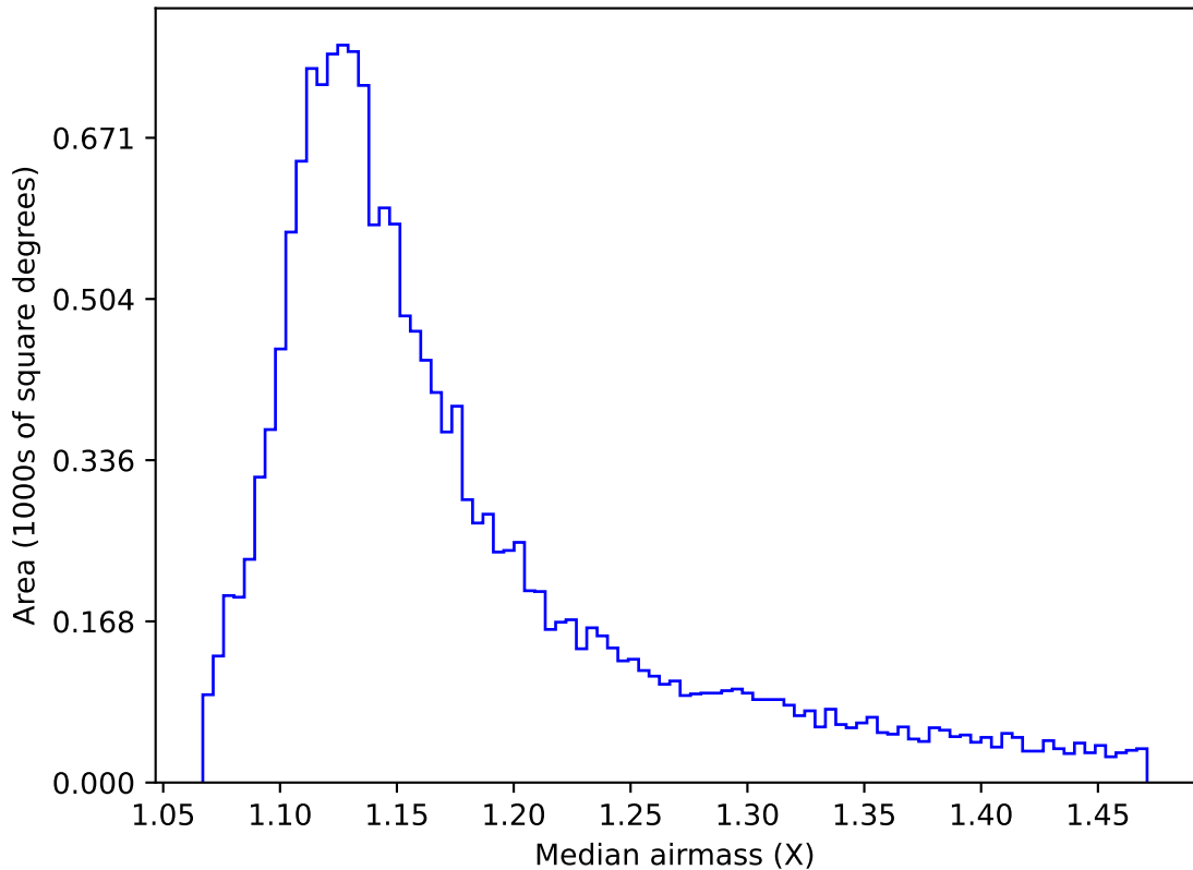
too_elab_r16_d2_ugrizy_v3.4_10yrs WFD u band: Median airmass
